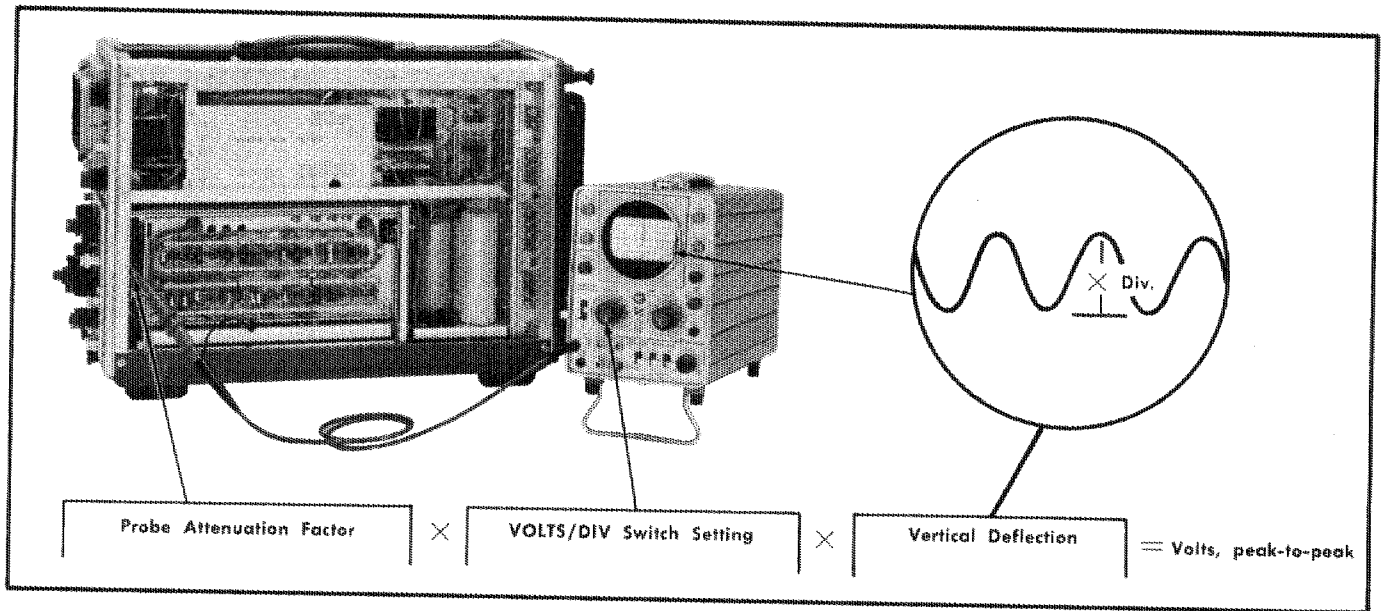
Fig. 3-8. Measuring the peak-to-peak ac voltage of an applied waveform.
